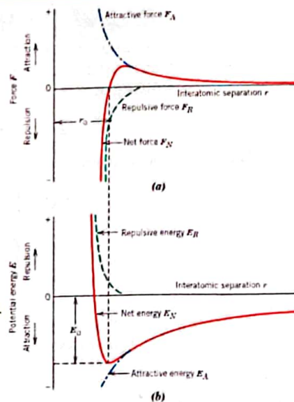
Fig. (a) The dependence of repulsive, attractive, and net forces on interatomic separation for two isolated atoms. (b) The dependence of repulsive, attractive, and net potential energies on interatomic separation for two isolated atoms.
