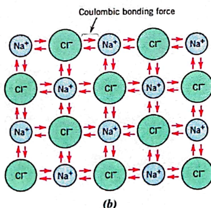
Figure 2.11 Schematic representations of (a) the formation of Na + and Cl - ions and (b) ionic bonding in sodium chloride (NaCl)
